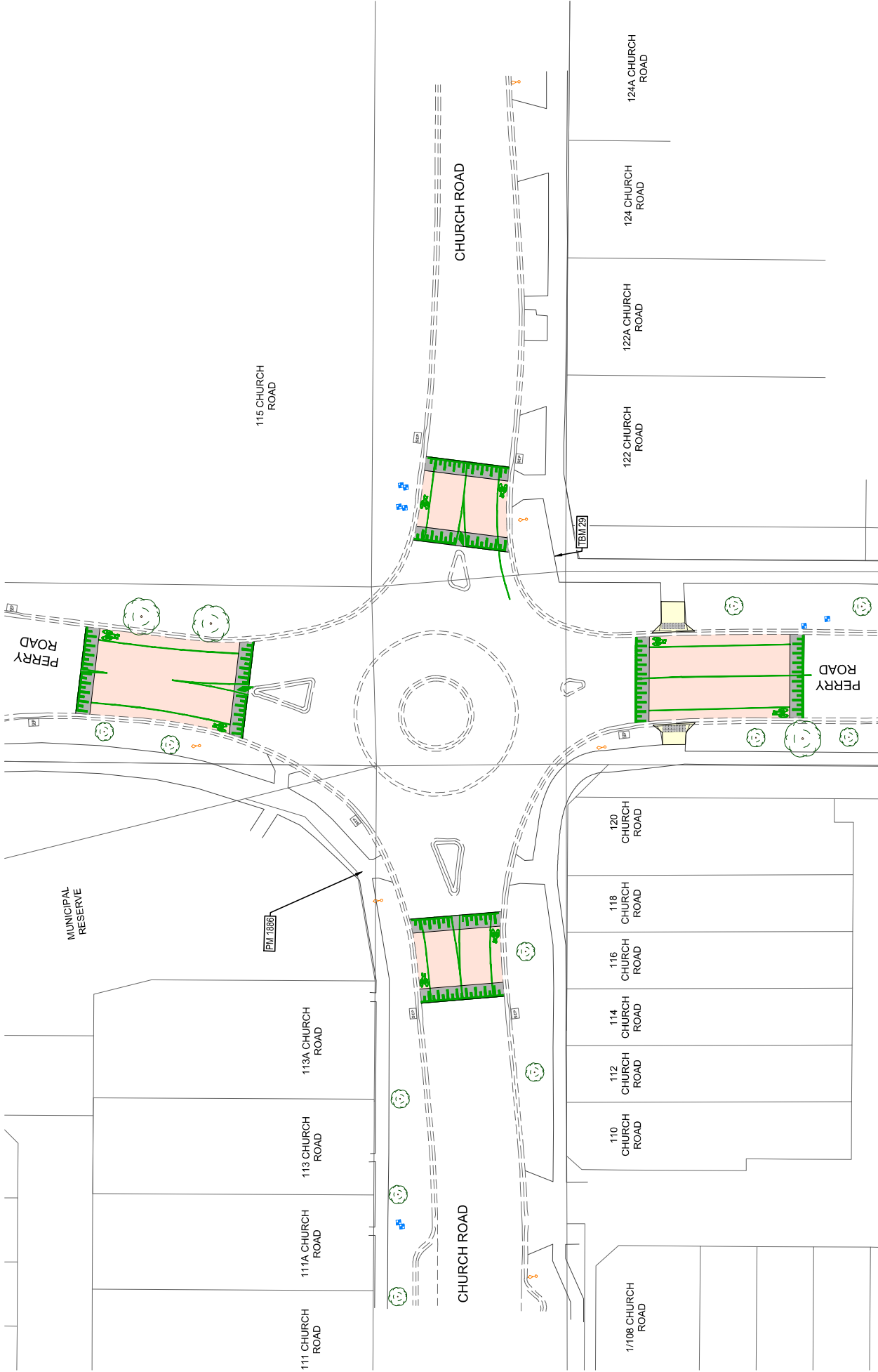
LAYOUT PLAN PERRY ROAD / CHURCH ROAD ROUNDABOUT
