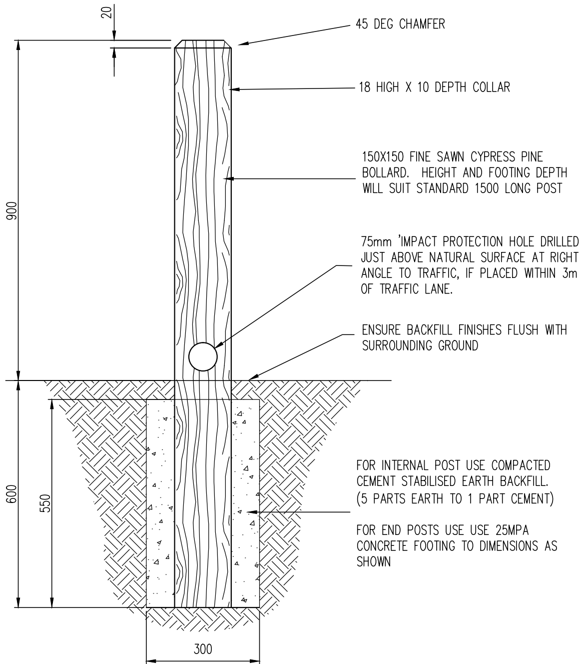
ELEVATION SCALE 1 : 10
