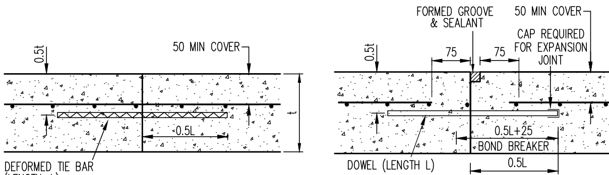
TIED JOINT NOT AT A CONTRACTION JOINT
