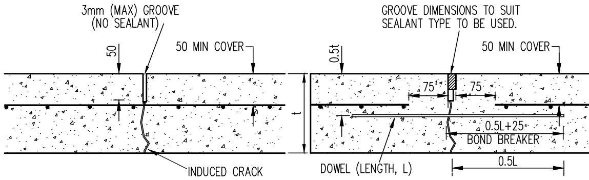
"INTERMEDIATE" SPACING 4m (MAX)
