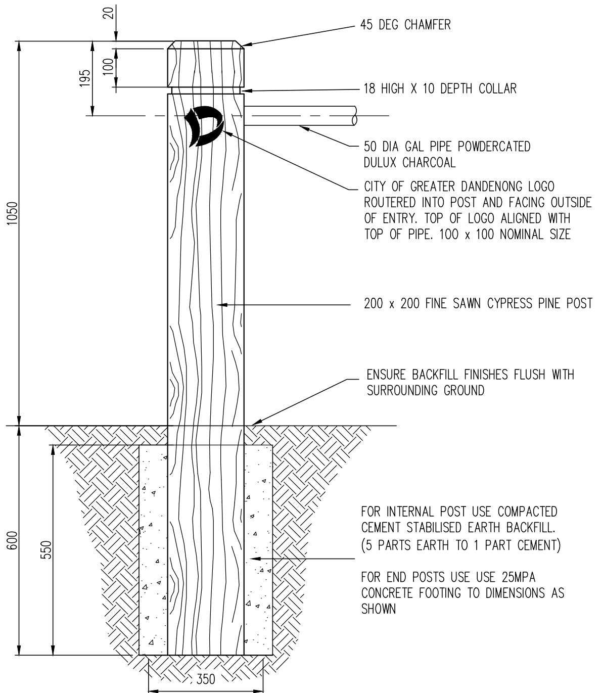
ELEVATION SCALE 1 : 10
