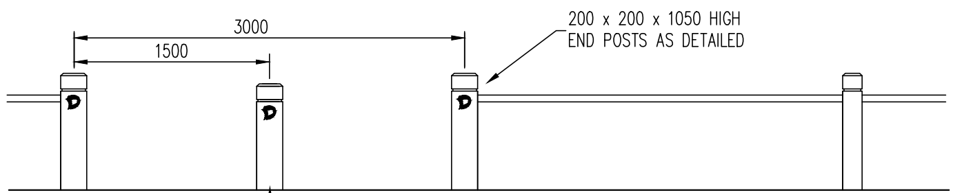
INSTALLATION ELEVATION SCALE 1 : 50
