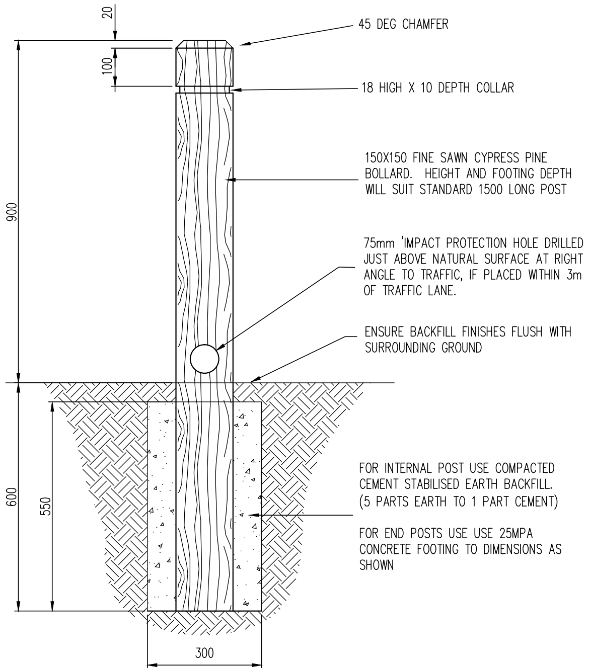
ELEVATION SCALE 1 : 10
